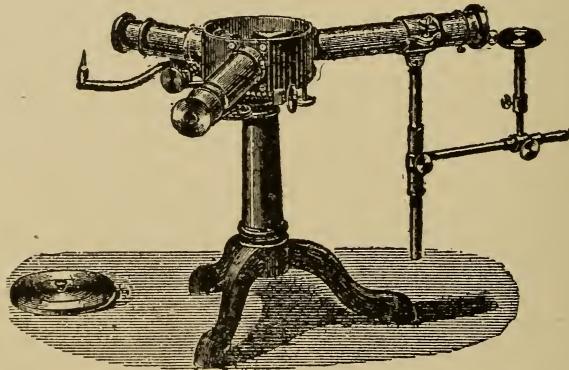
Fig. 73. A SPECTROSCOPE.
